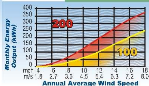
Rayleigh Distribution Curve k=2
