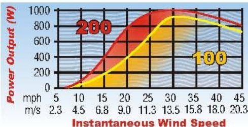
Performance Curves
